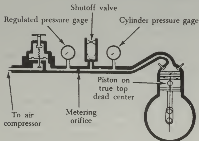
FIGURE 10-46. Differential compression tester.
